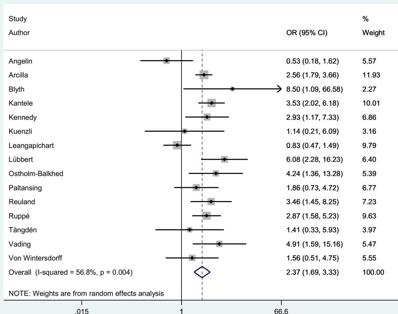
Figure 2: Forest plot of random effects model, for odds ratio (OR) of extended-spectrum beta-lactamase-producing Enterobacteriaceae (ESBL-PE) among participants exposed to, compared to those not exposed to, antimicrobials during travel
