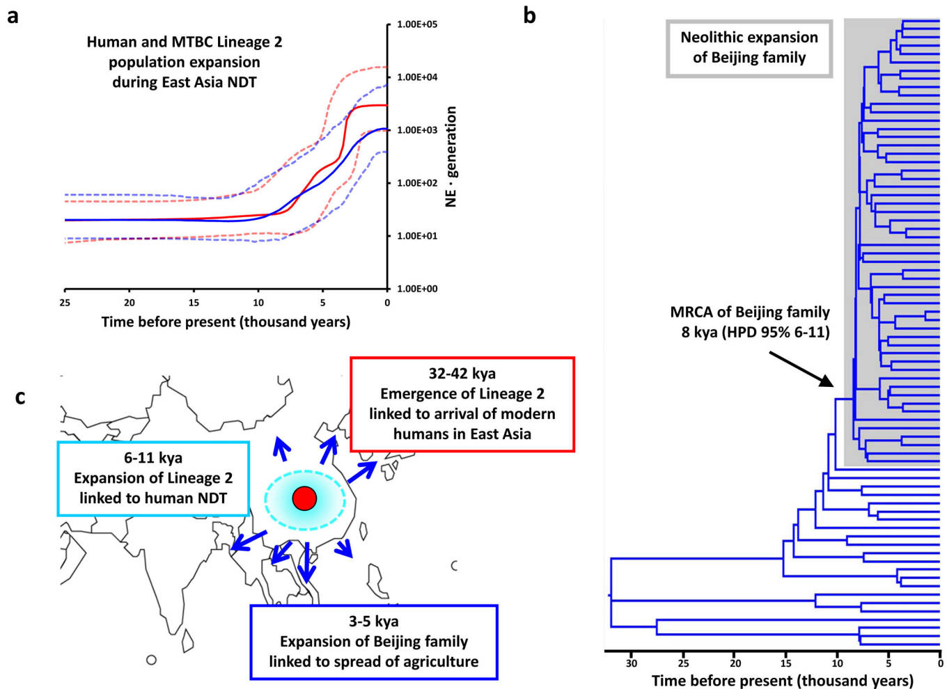
Figure 3. Neolithic expansion and spread of MTBC Lineage 2 “Beijing” in East Asia
