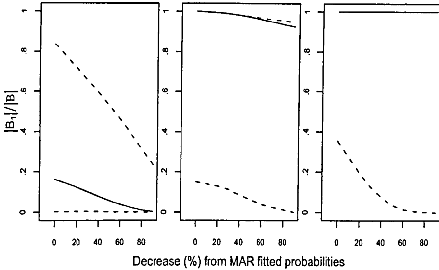
Figure 6.2: Weighted proportions (solid lines) of estimates of \beta_1 in (6.9) that are greater than zero over all possible sample completions when the values of p_i in (6.8) vary in the range shown on the x-axis. Dotted lines represent 95% bootstrap confidence intervals. Simulated data (ii) to (iv) are shown from left to right.
