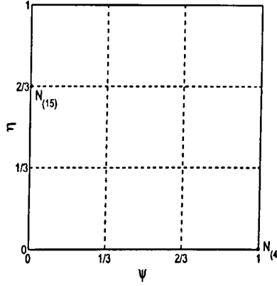
Figure 4.6: Grid of nodal points for 2-dimensional Lagrangian interpolation cubic in each coordinate.
