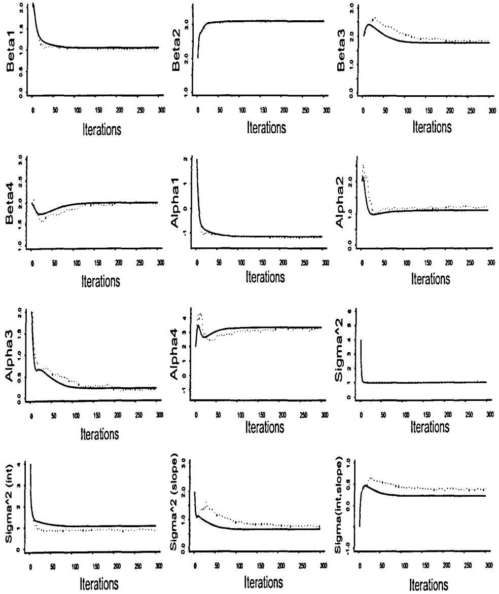
Figure 3.5: Sequences of parameter estimates for models (3.9) and (3.10) jointly fitted using a MCEM algorithm (dotted line) and a quasi-MCEM algorithm (solid line).
