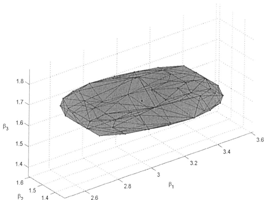
Figure 5.4: Region of ignorance for parameters \beta_1 , \beta_2 and \beta_3 in (5.9) when each missing measurement is allowed to take value in the interval defined as \hat{y}_{ij} \pm 0.5\hat{\sigma}^2 (Scenario A). \hat{y}_{ij} and \hat{\sigma}^2 are the predicted values for the mean of the missing observations and the estimated variance of the error term, respectively, from the fit of (5.9) to the available cases.
