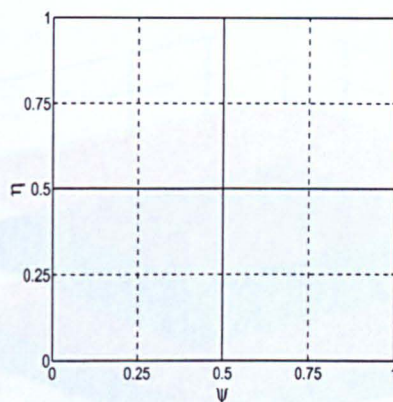
Figure 4.8: Application to the Parkinson's disease trial: grid of nodal points for 2-dimensional Lagrangian interpolation quadratic in each coordinate.
